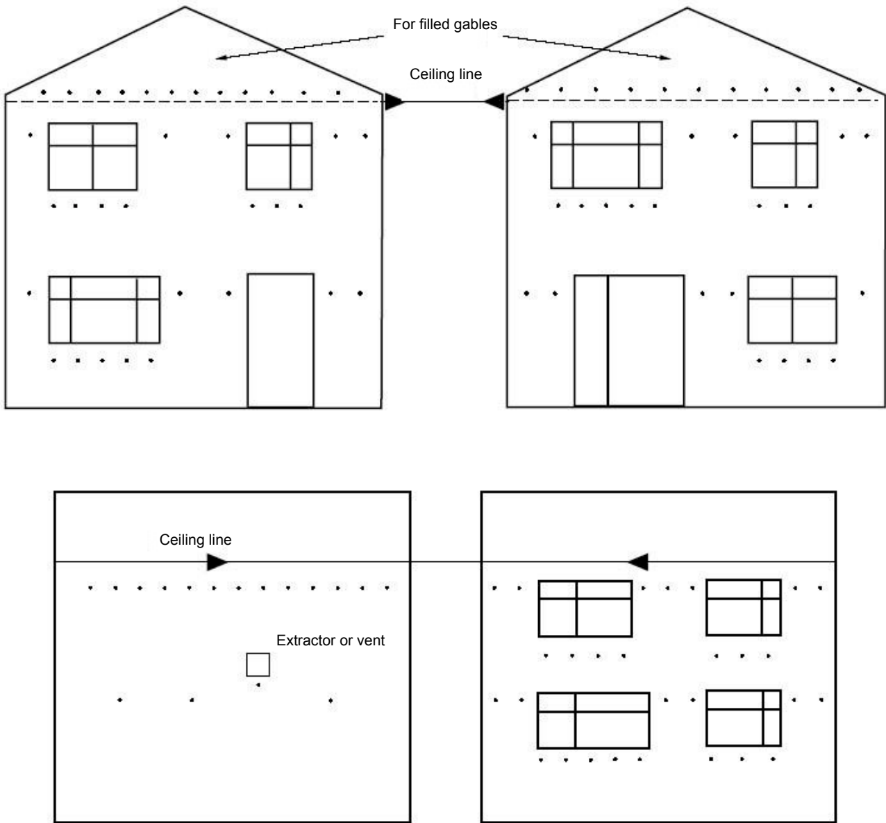
Figure 1: Typical EcoBead / EcoBead Platinum Hole Drilling Pattern in a Detached Dwelling
